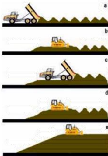
Figure 5-2. Stockpiling dry non-plastic soils
