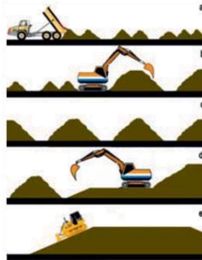
Figure 5-3 Stockpiling wet plastic soils.
